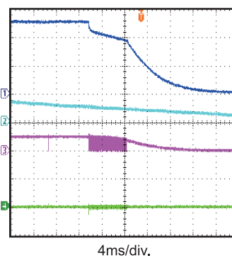
Shut Down Through V_{IN} V_{IN}=22V , I_{OUT} = 0A
